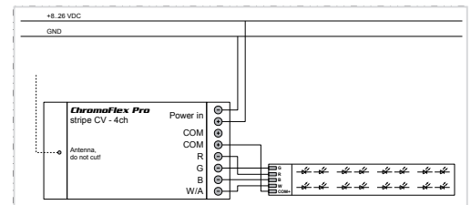
Anschlusskizze 4-Kanal connection drawing 4 channel
