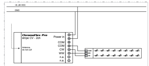
Anschlusskizze 2-Kanal connection drawing 2 channel
